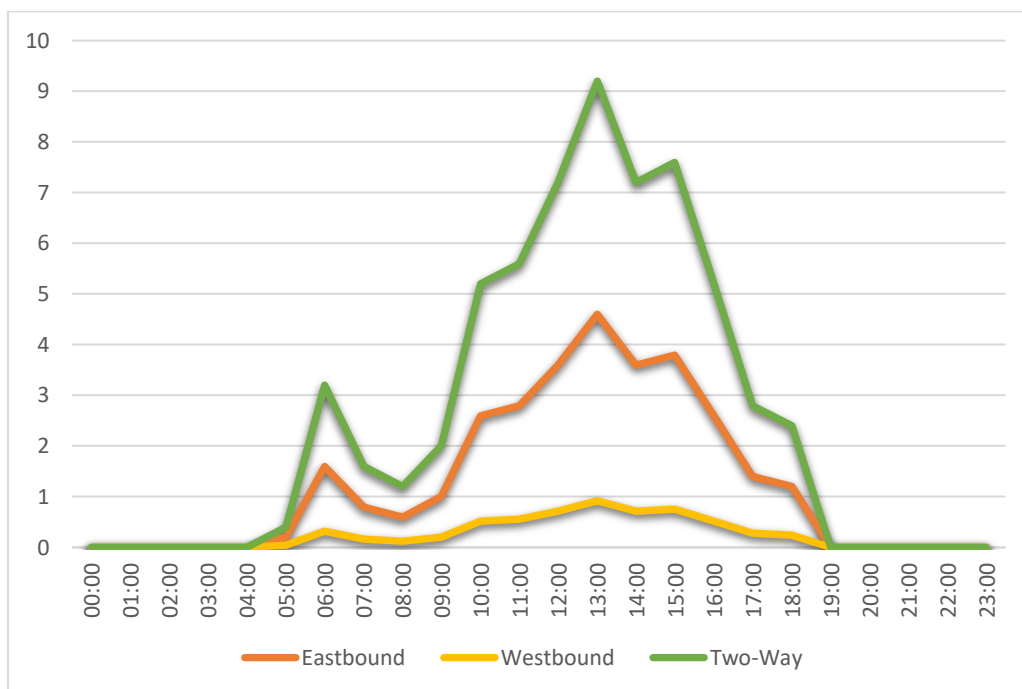
Figure 4: L5252 Traffic Profile
