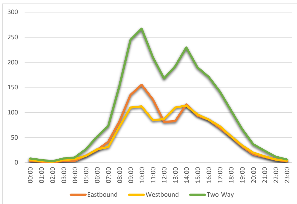
Figure 2: N59 Traffic Profile
