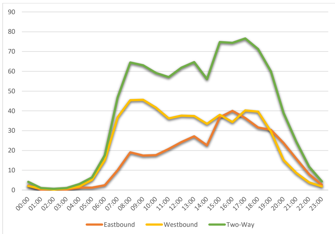
Figure 3: L1206 Traffic Profile
